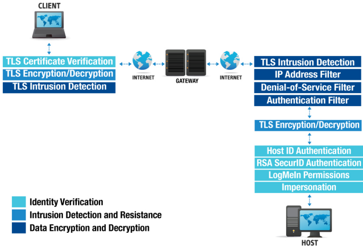
Figure 4: Authentication between Users and the Host
